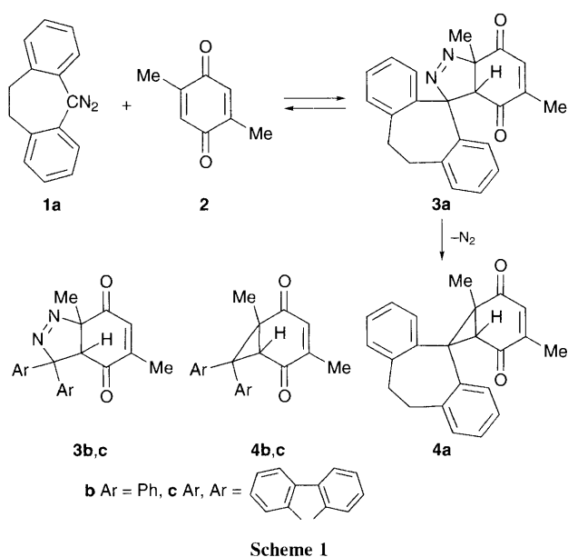
Fig. 1 Molecular structure and atom labelling scheme of 3a . Selected bond lengths (Å) and angles (°): O(2)–C(4), 1.217(9); O(1)–C(1), 1.218(9); N(1)–N(2), 1.247(8); N(1)–C(5), 1.515(9); N(2)–C(9), 1.511(8); C(5)–C(6), 1.519(9); C(6)–C(9), 1.580(9); C(9)–C(10), 1.546(9); C(9)–C(23), 1.539(9); C(10)–C(15), 1.380(9); C(15)–C(16), 1.514(10); C(16)–C(17), 1.540(11); C(17)–C(18), 1.519(10); C(18)–C(23), 1.401(9); N(2)–N(1)–C(5), 112.6(6); N(1)–N(2)–C(9), 112.9(6); N(1)–C(5)–C(6), 105.6(5); C(5)–C(6)–C(9), 102.5(5); N(2)–C(9)–C(10), 106.0(5); N(2)–C(9)–C(23), 105.3(5); C(9)–C(10)–C(15), 126.4(6); C(9)–C(23)–C(18), 120.9(6); C(10)–C(15)–C(16), 126.8(6); C(15)–C(16)–C(17), 116.2(6); C(16)–C(17)–C(18), 110.3(6); C(17)–C(18)–C(23), 120.7(6).
